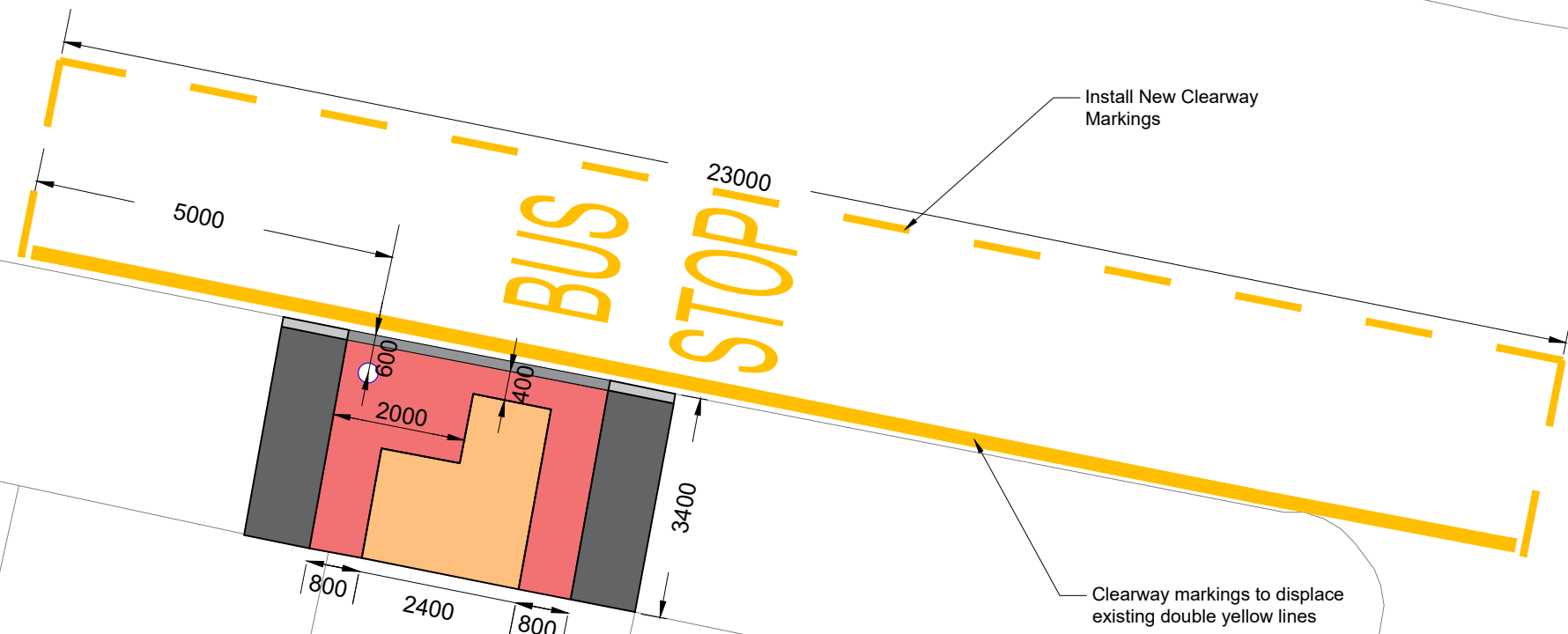
Bus Stop General Arrangement UPBS05 Scale 1:100
